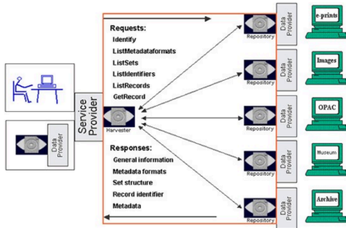
14 Figure 4 - Sample OAI Request Encoding
