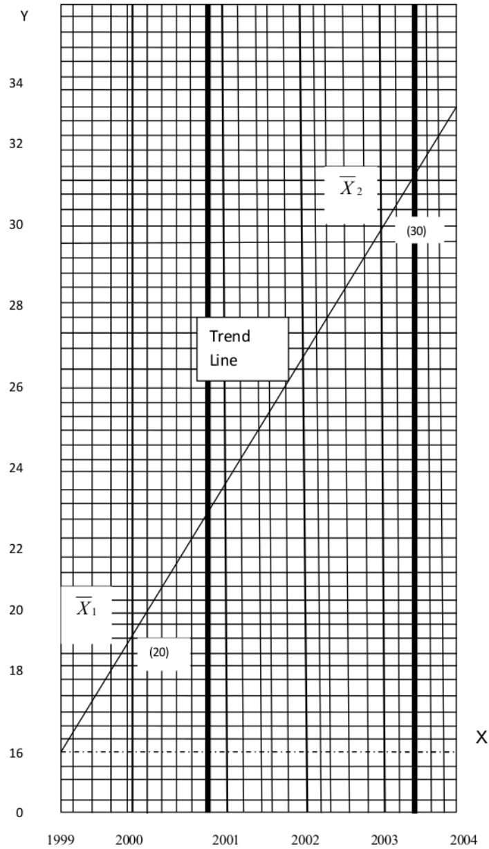
Graphic representation of the trend line by the method of semi averages.
