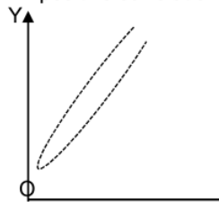
High degree of positive correlation
